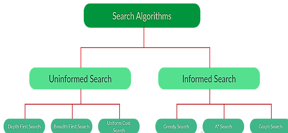
Fig. 1. Search algorithm [16].
