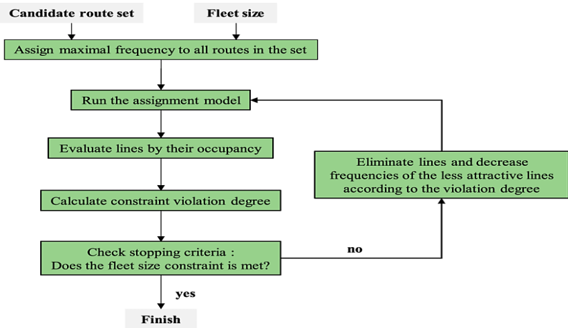
Fig. 4. Heuristics algorithms [22].
